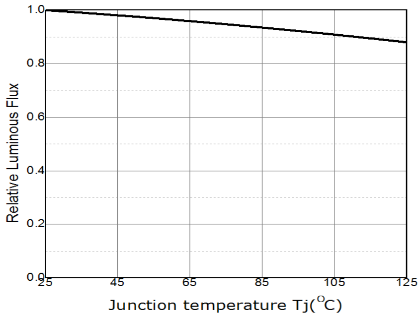
Fig 6. Junction Temperature vs. Relative Luminous Flux, I_F=120\text{mA}
