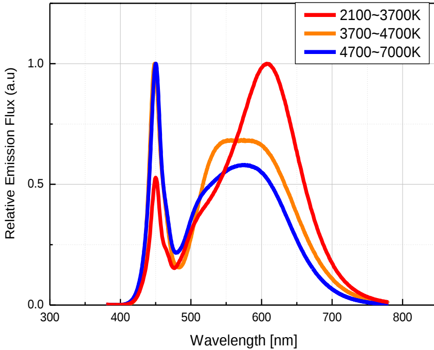
Fig 1. Color Spectrum, T_j = 25^\circ\text{C} , I_F = 120\text{mA}
