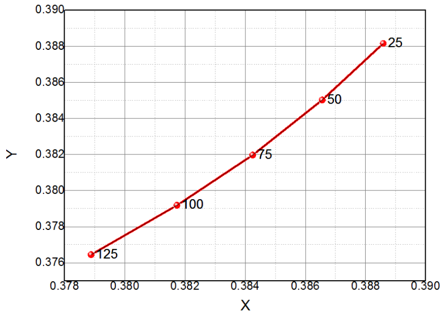
Fig 8. Chromaticity Coordinate vs. Junction Temperature, I_F=120\text{mA} (2600~4200K)
