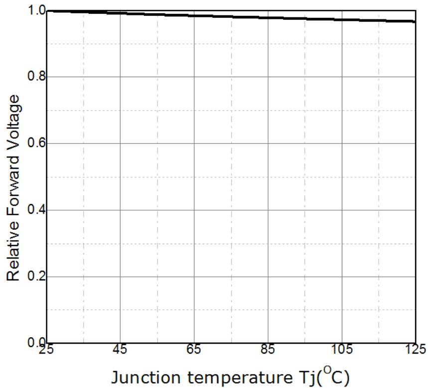
Fig 7. Junction Temperature vs. Relative Forward Voltage, I_F=120\text{mA}
