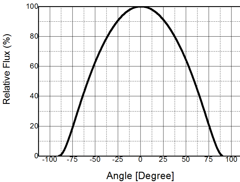
Fig 2. Radiant Pattern, T_j = 25^\circ\text{C} , I_F = 120\text{mA}
