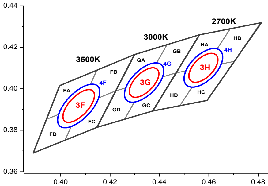
CIE Chromaticity Diagram T_j=25^{\circ}\text{C} , I_F=120\text{mA}
